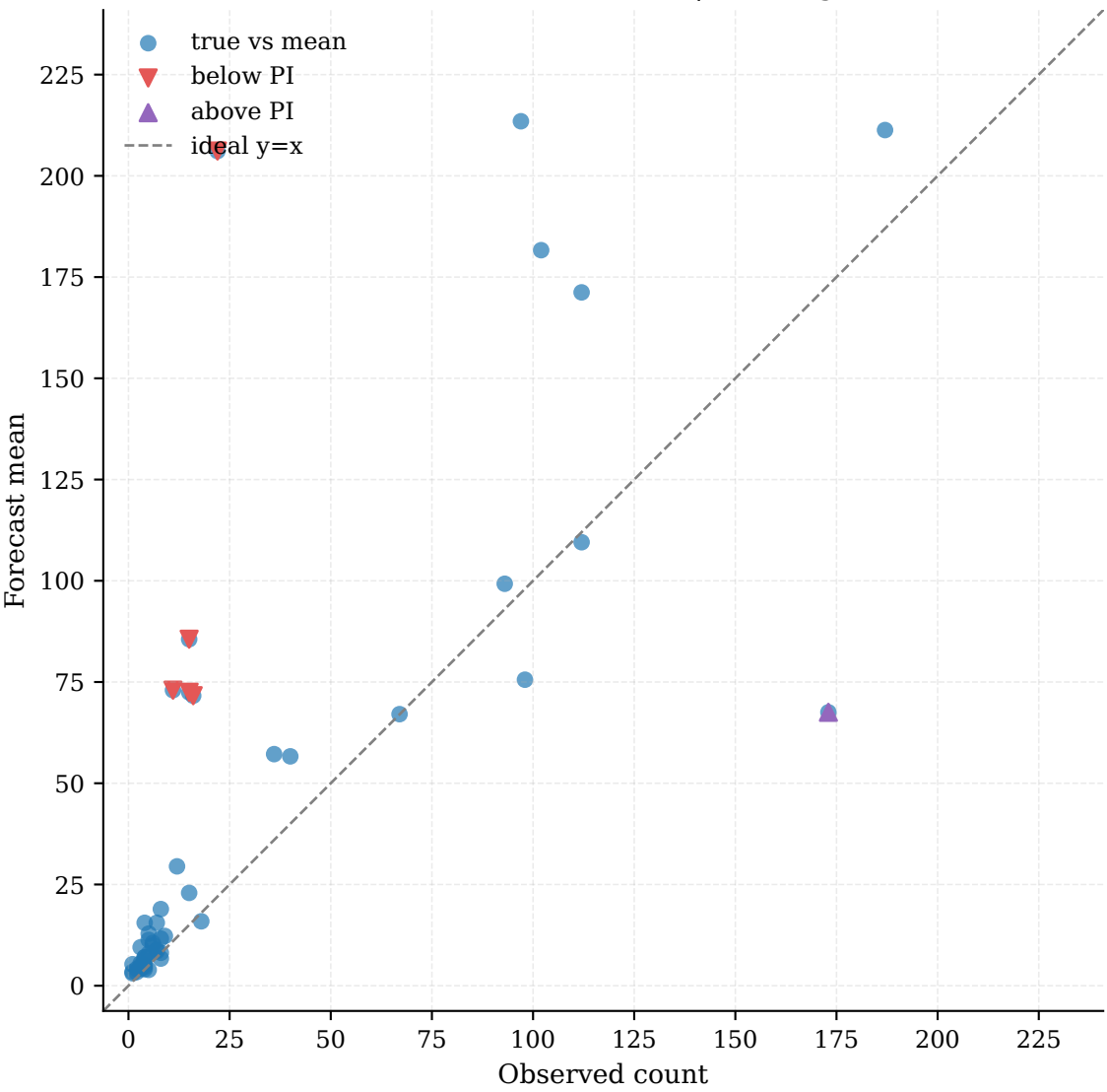
Observed vs Forecast (zoomed) | Coverage: 80.33%
