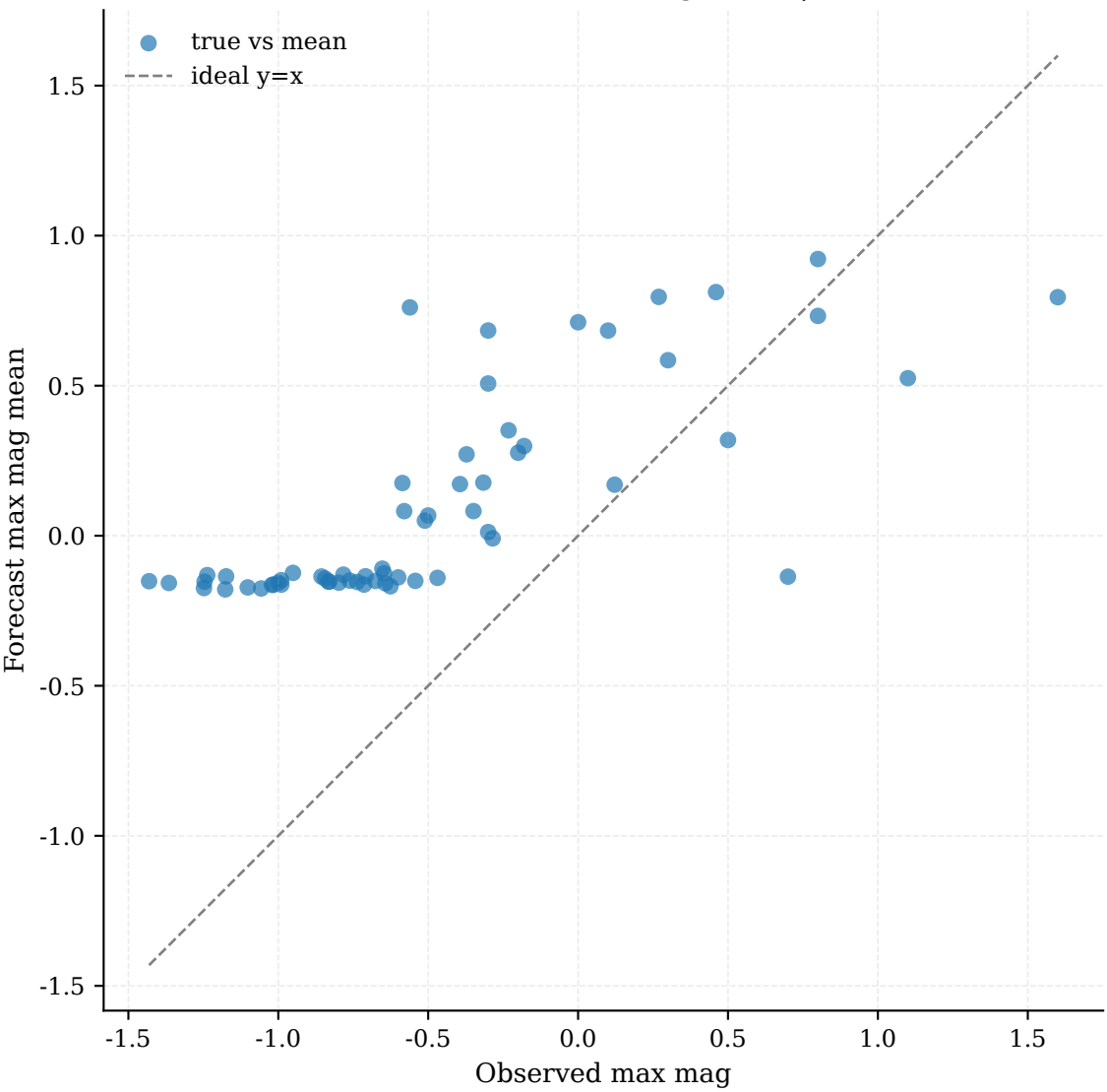
Observed vs Forecast Max Magnitude | MAE: 0.65
