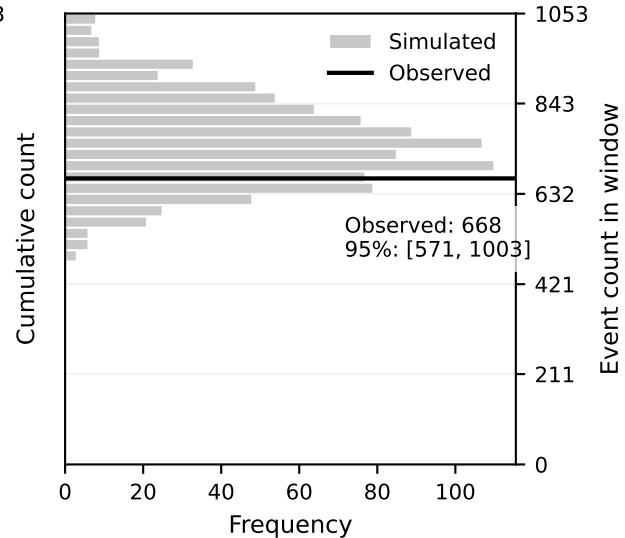
Forecast counts
