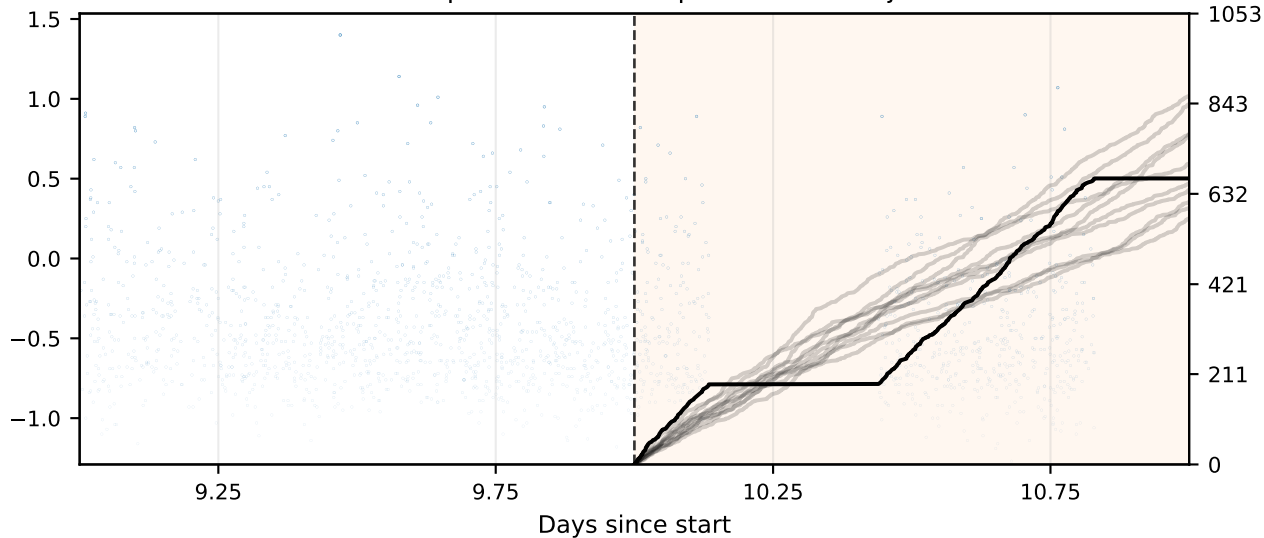
Observed Sequence and Example Forecast Trajectories
