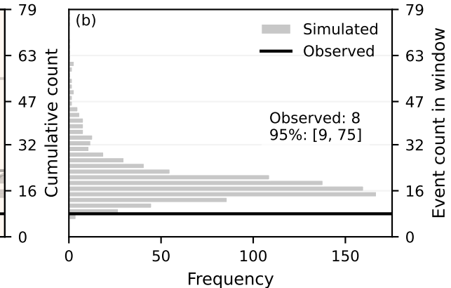
Forecast counts
