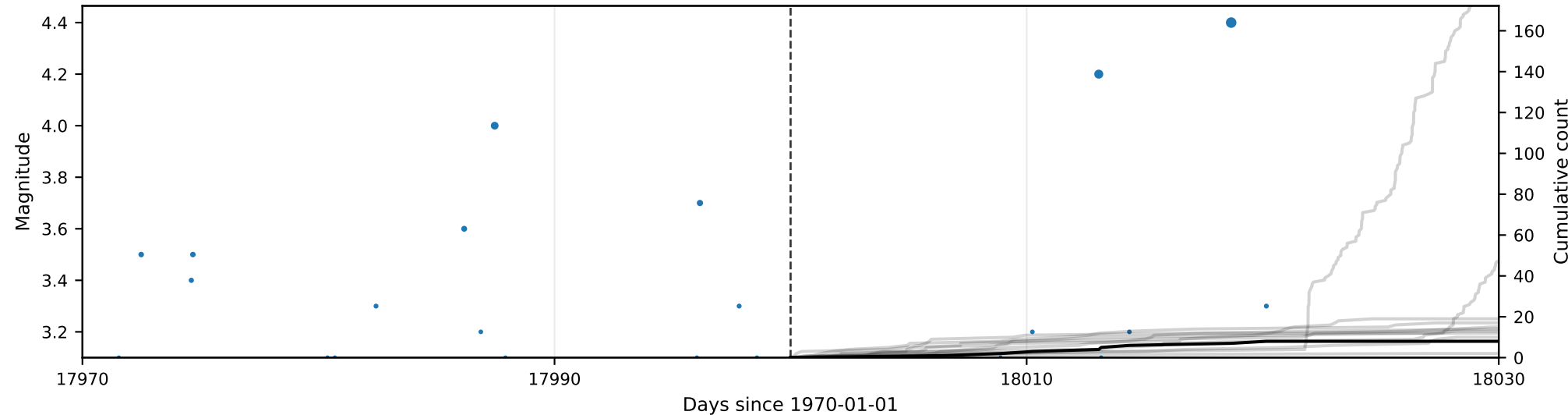
Observed sequence + example forecast trajectories
