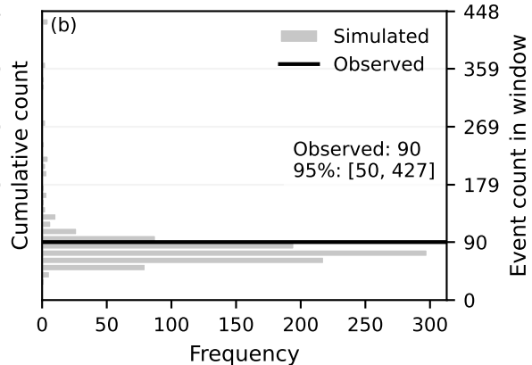
Forecast counts
