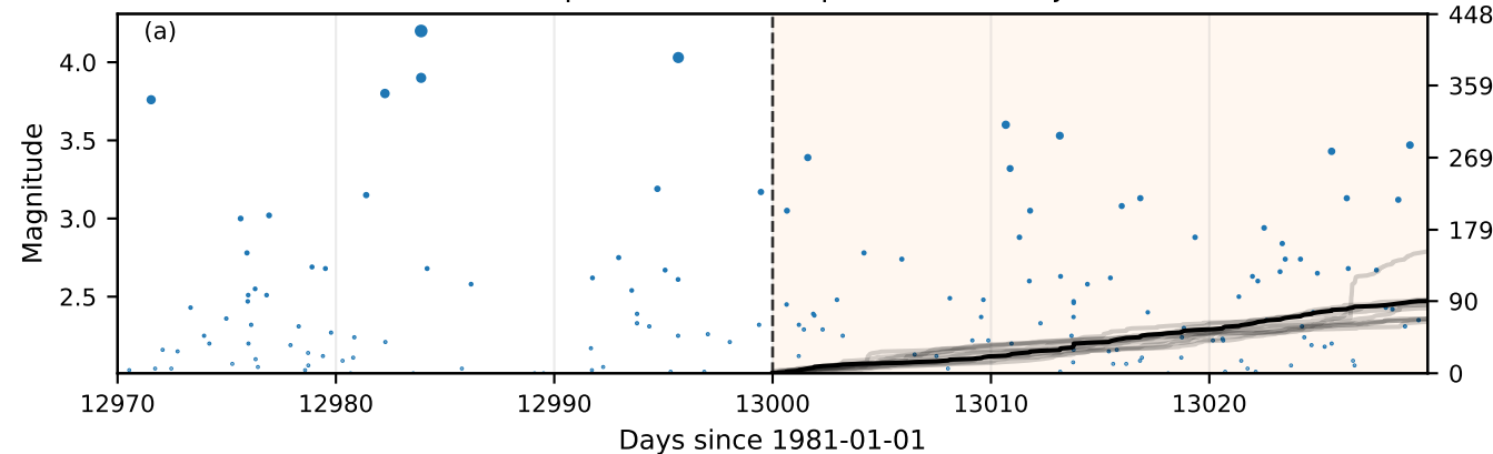
Observed Sequence and Example Forecast Trajectories
