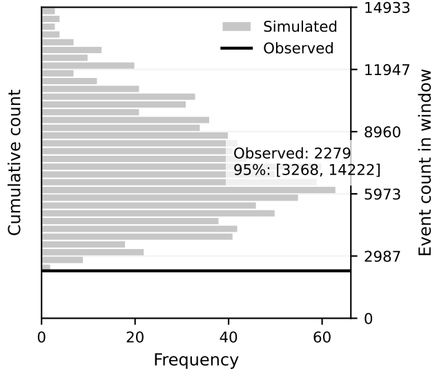
Forecast counts
