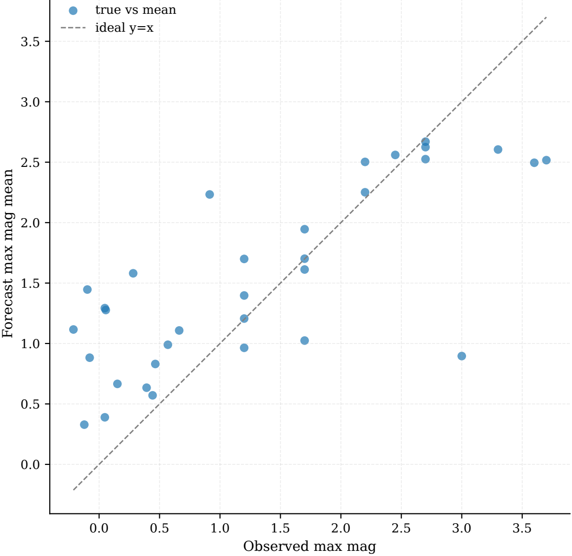
Observed vs Forecast Max Magnitude | MAE: 0.59
