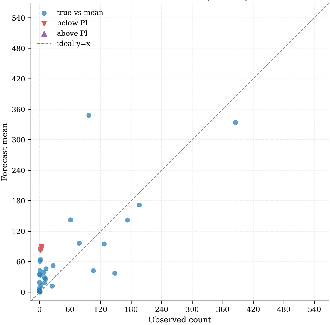
Observed vs Forecast (zoomed) | Coverage: 95.45%
