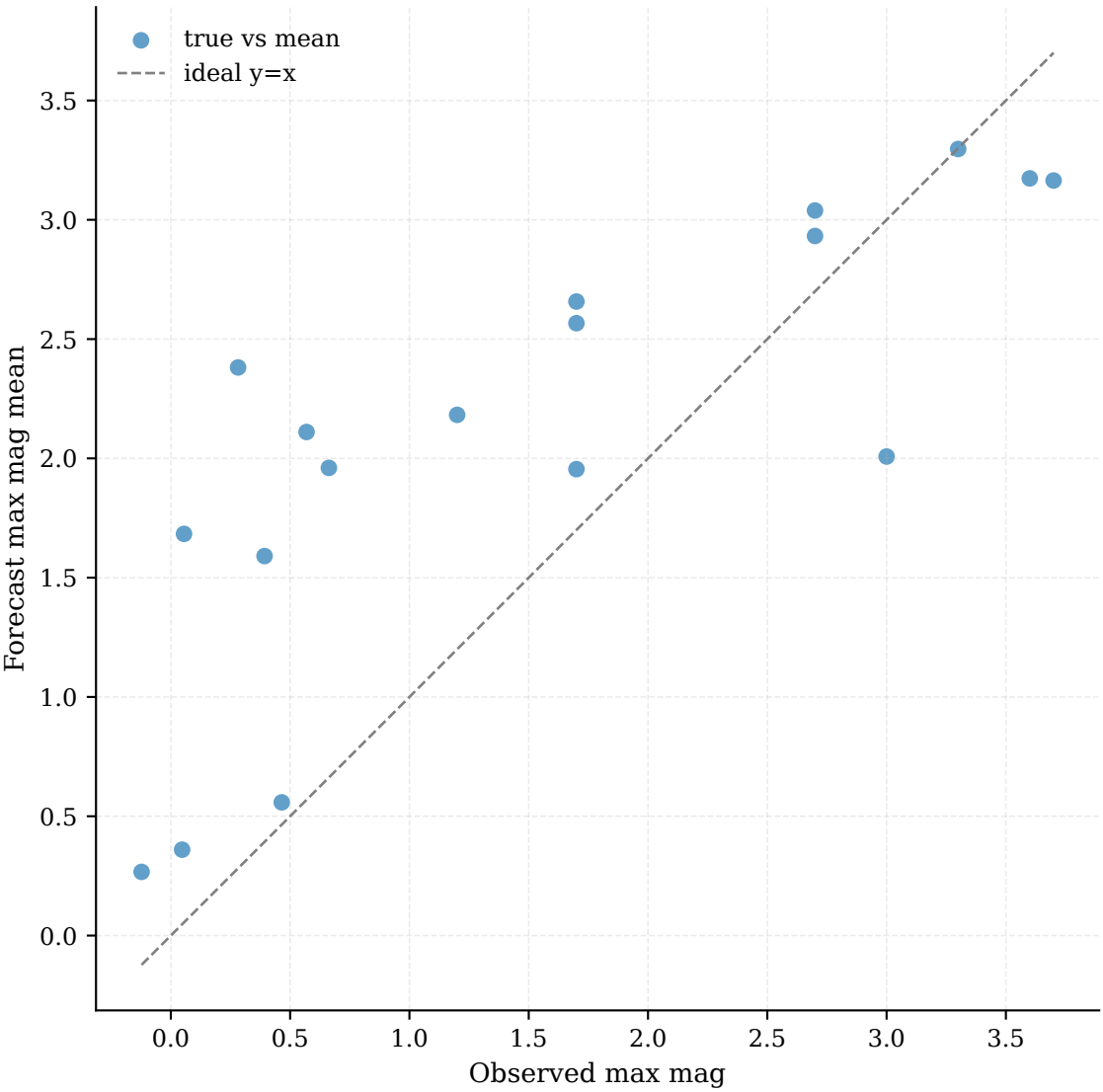
Observed vs Forecast Max Magnitude | MAE: 0.79
