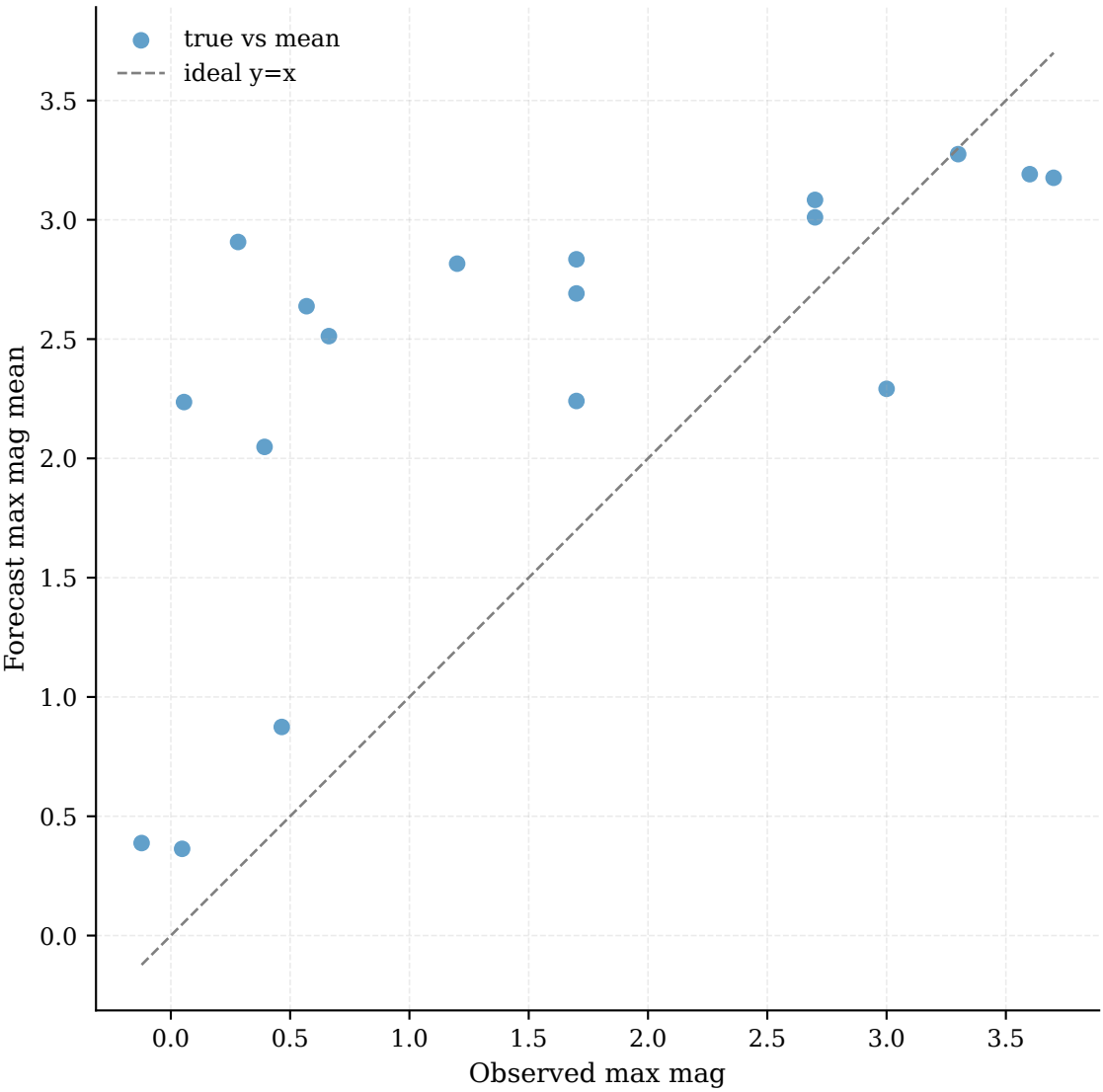
Observed vs Forecast Max Magnitude | MAE: 1.01
