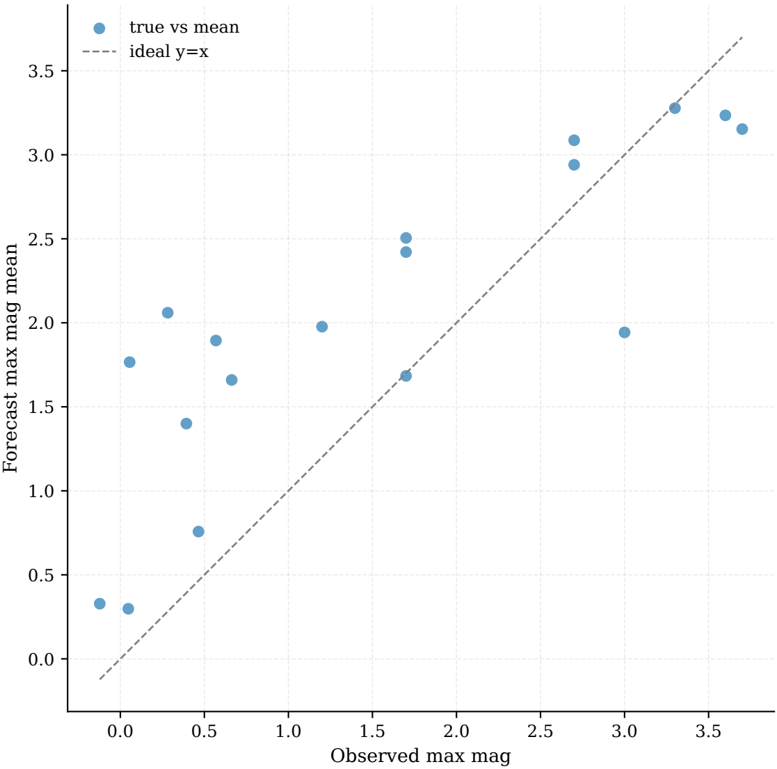
Observed vs Forecast Max Magnitude | MAE: 0.71
