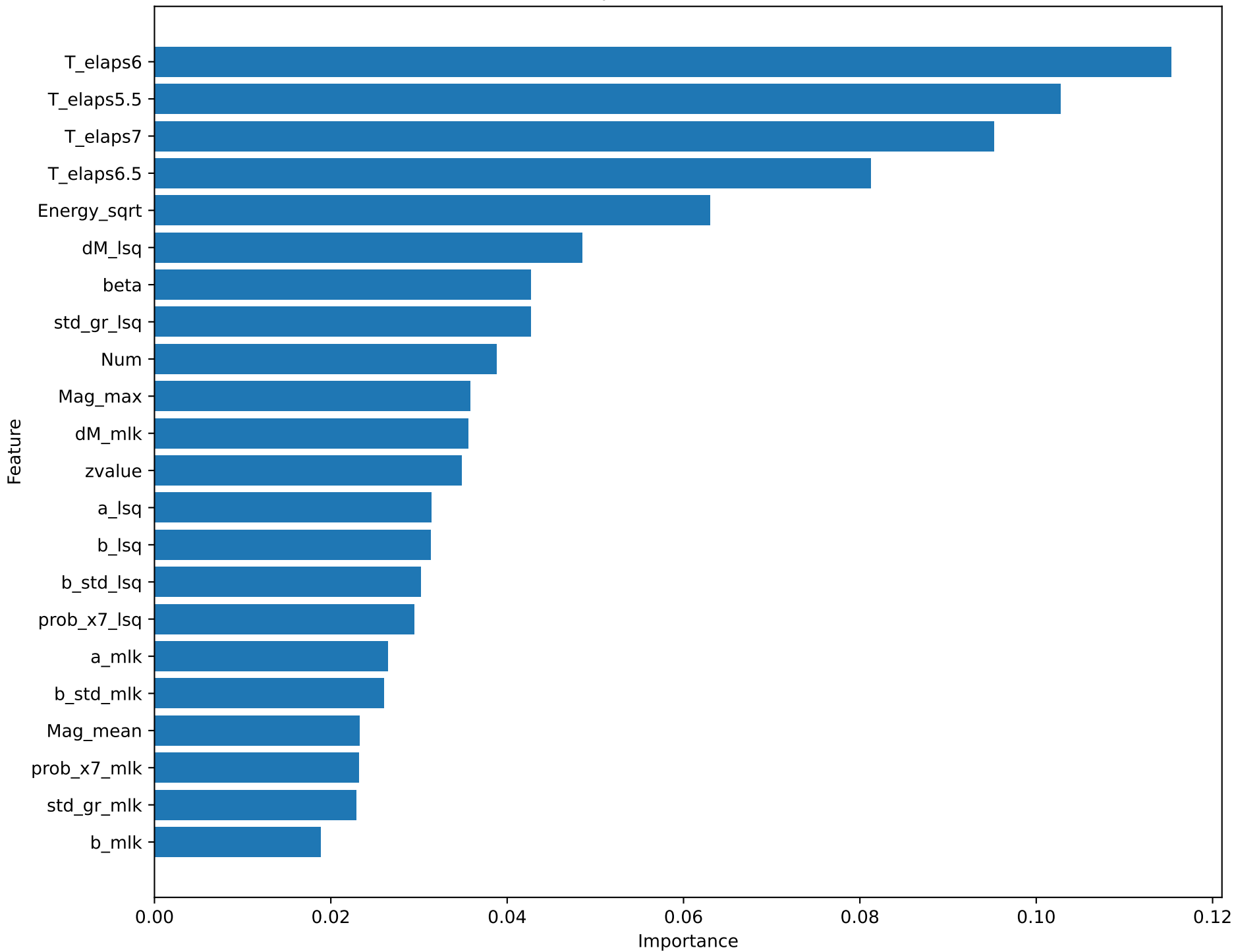
Feature Importances (Random Forest)
