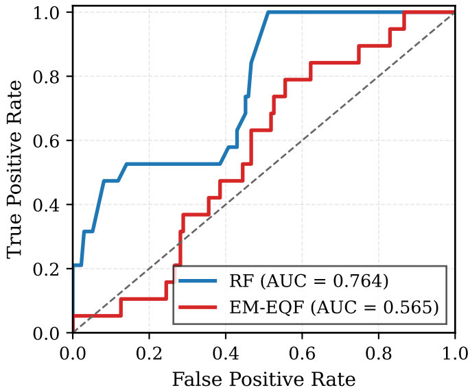
ROC Curve
