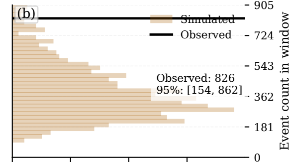
Forecast counts
