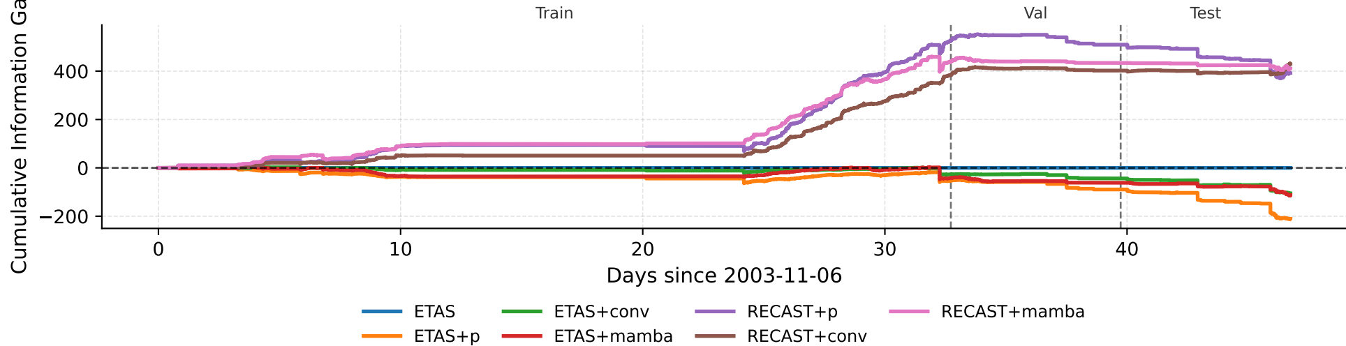
Cumulative log-likelihood difference over time
