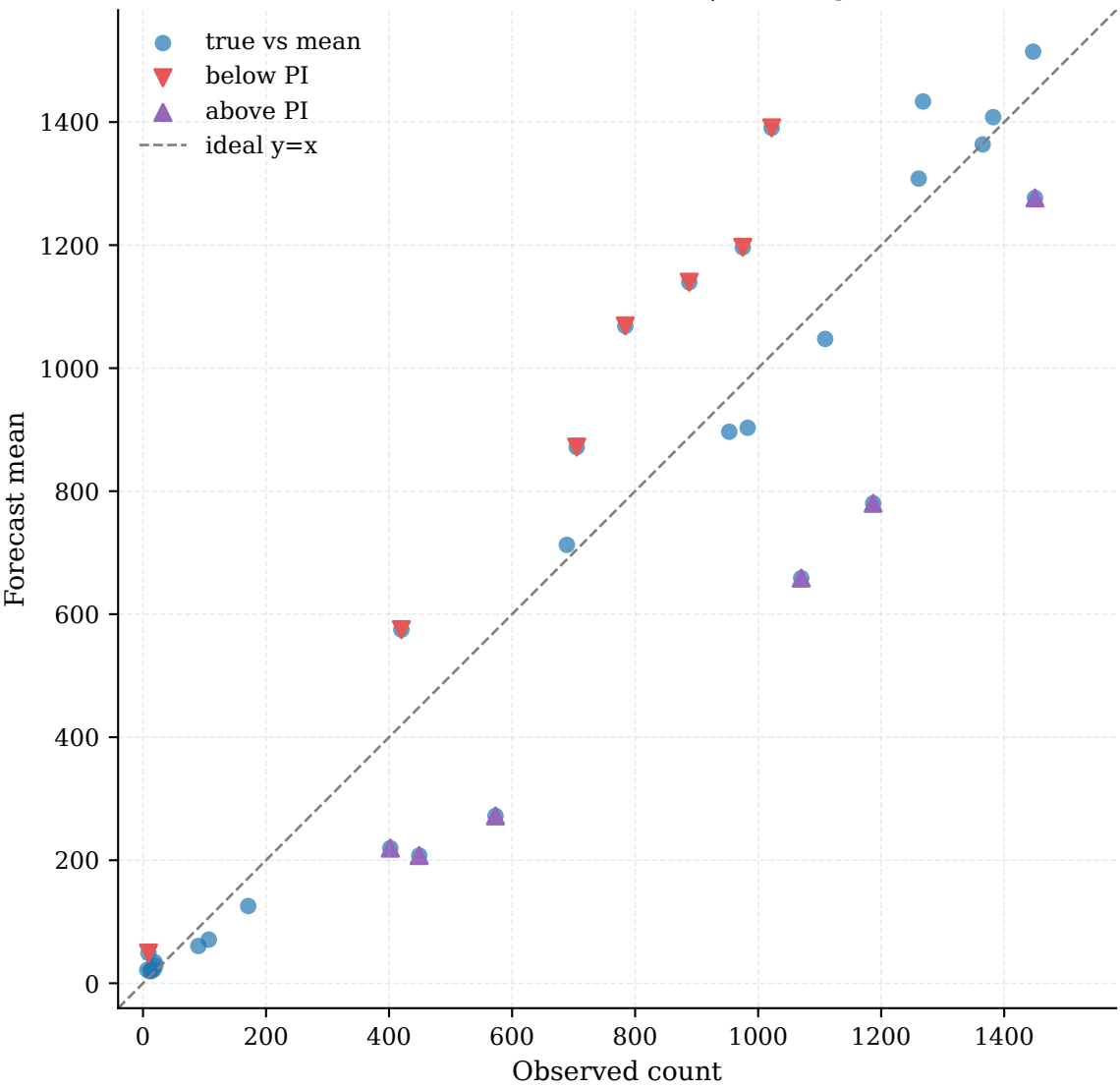
Observed vs Forecast (zoomed) | Coverage: 63.89%
