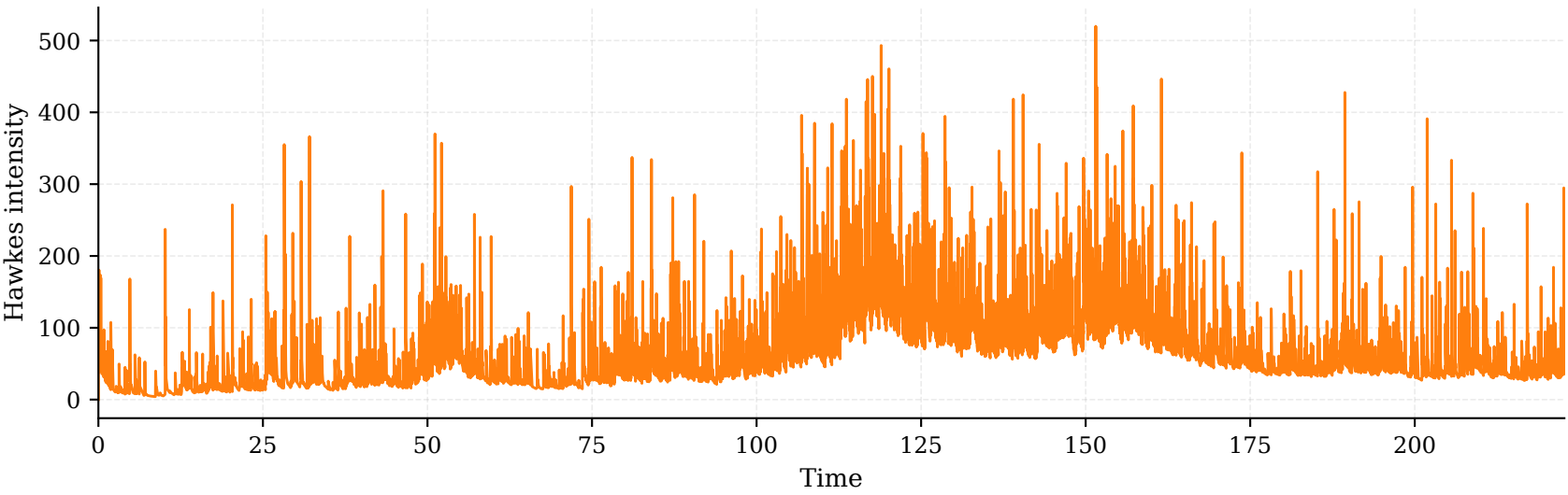
Hawkes Intensity
