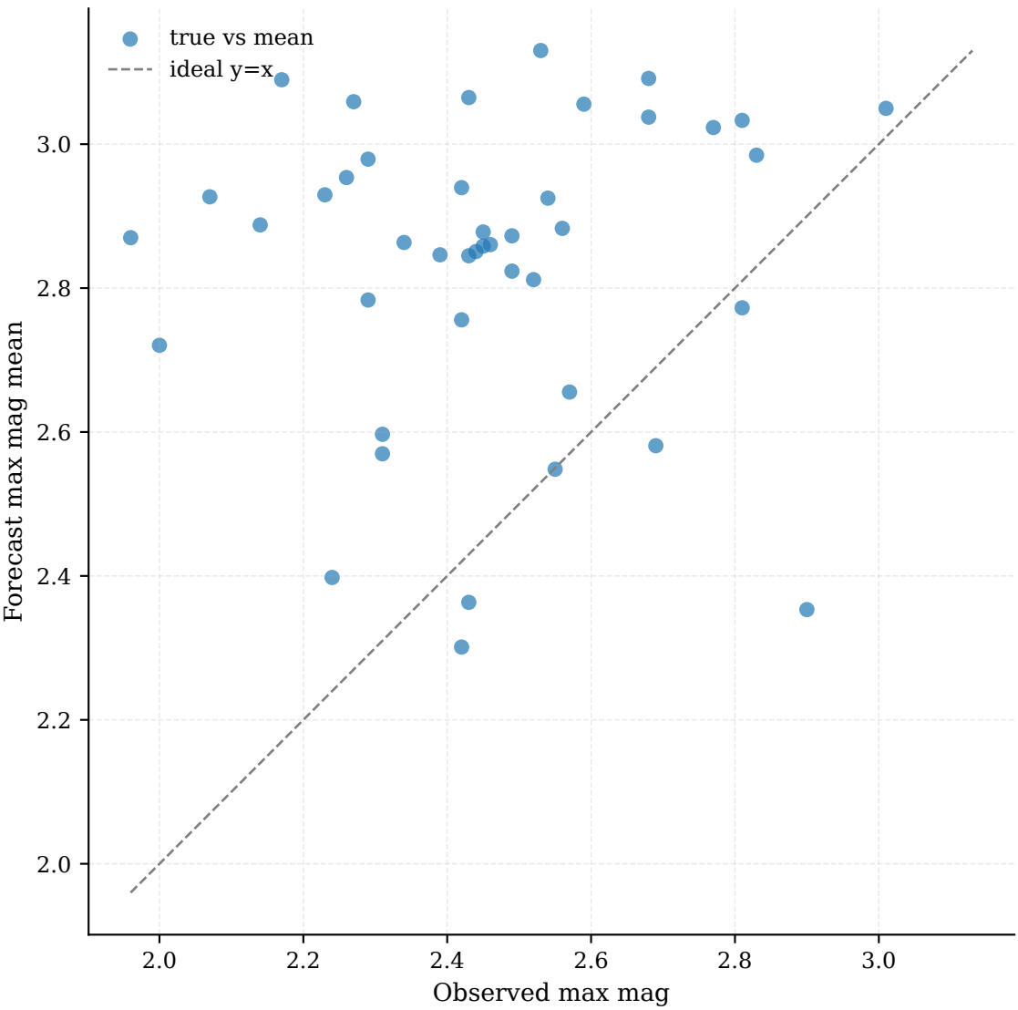
Observed vs Forecast Max Magnitude | MAE: 0.42
