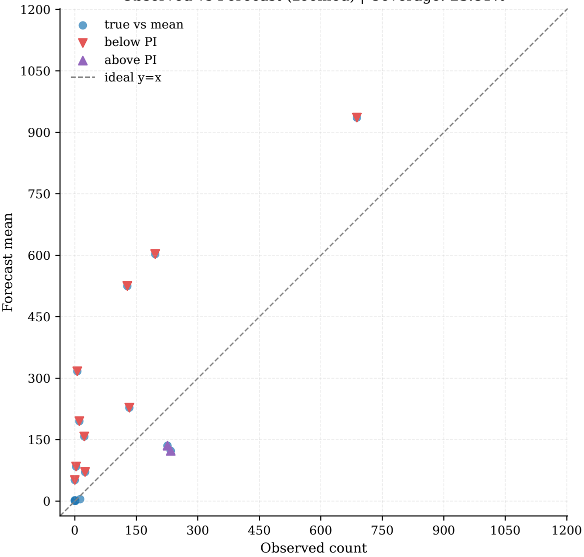
Observed vs Forecast (zoomed) | Coverage: 23.81%
