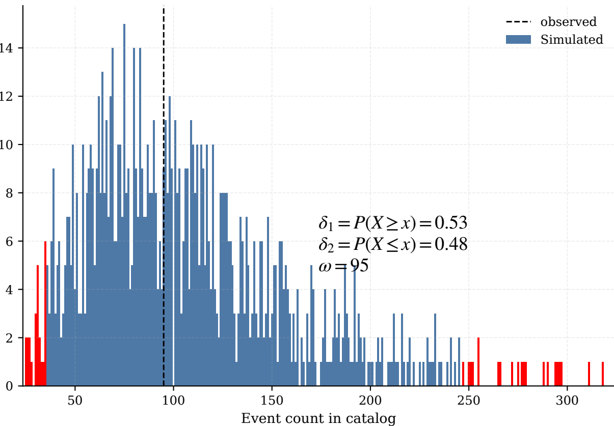
N-Test: Observed vs Simulated Event Counts
