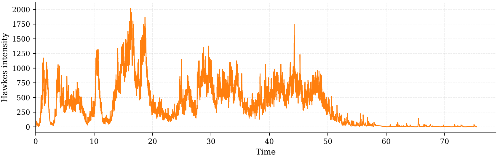
Hawkes Intensity
