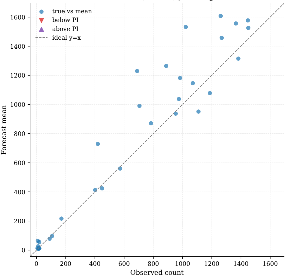
Observed vs Forecast (zoomed) | Coverage: 100.00%
