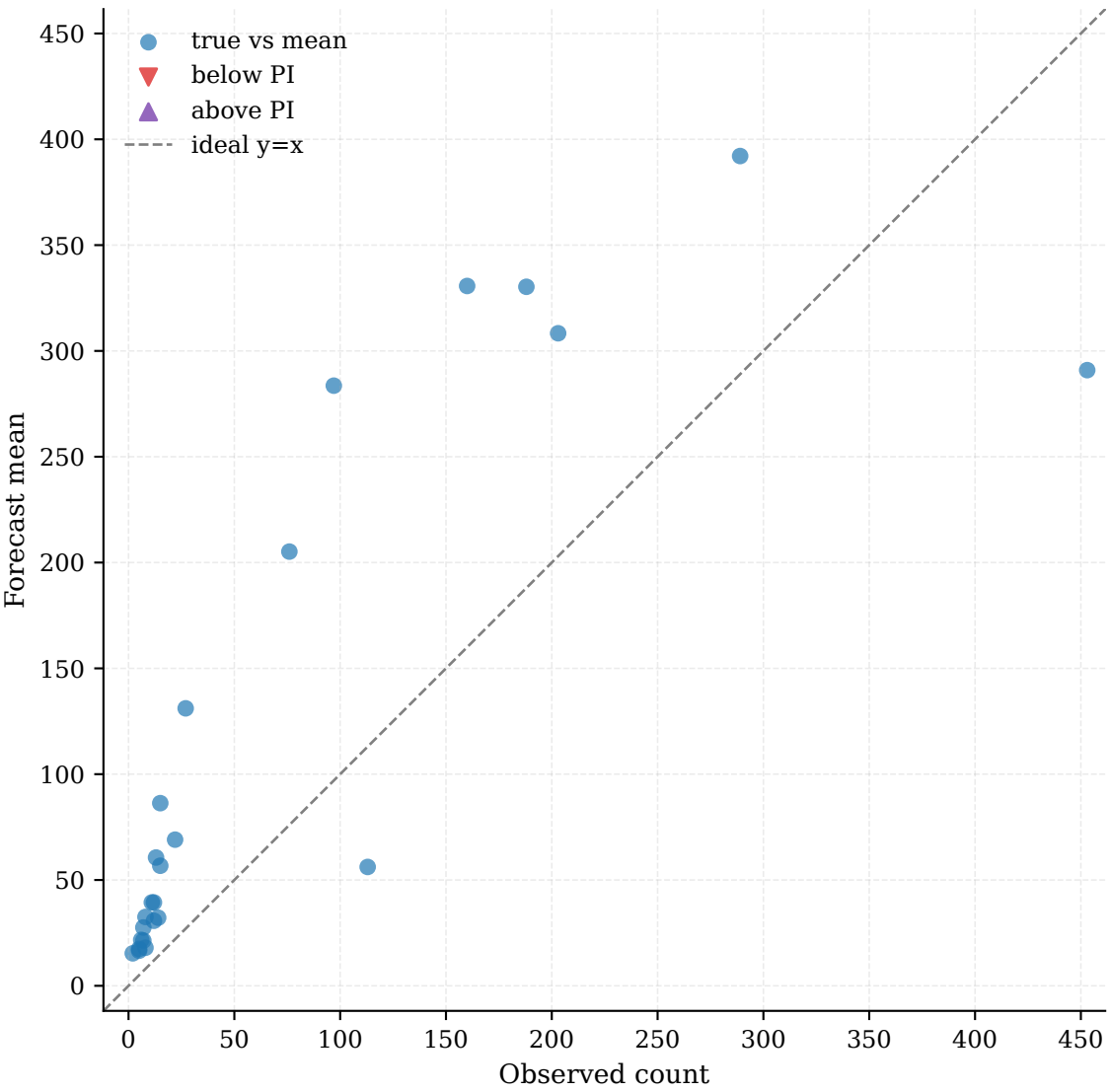
Observed vs Forecast (zoomed) | Coverage: 93.33%
