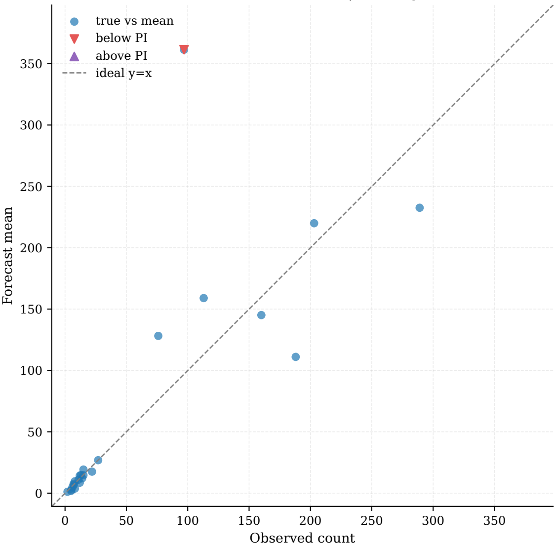
Observed vs Forecast (zoomed) | Coverage: 76.67%
