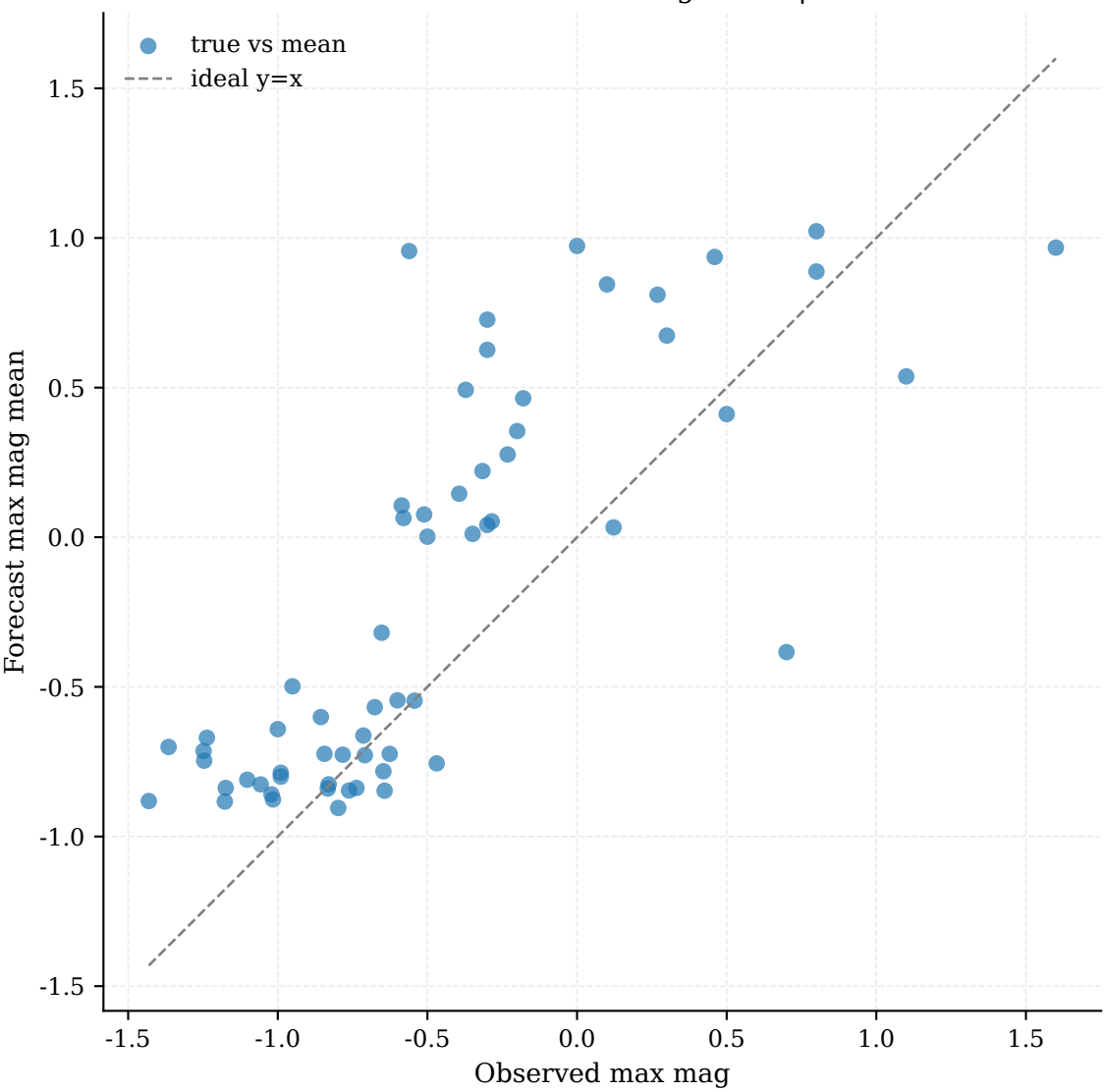
Observed vs Forecast Max Magnitude | MAE: 0.39
