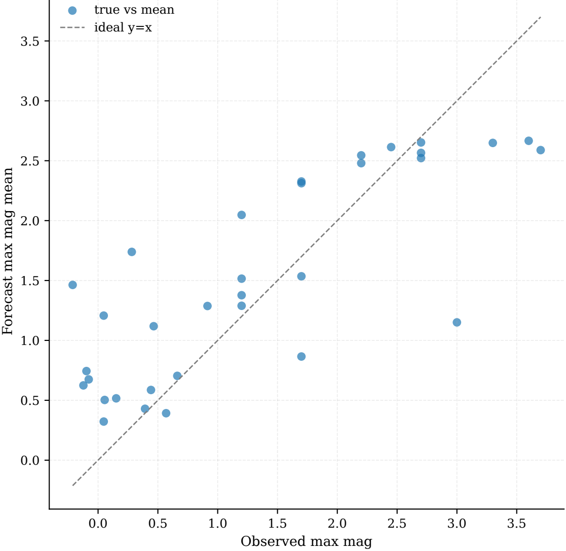
Observed vs Forecast Max Magnitude | MAE: 0.56
