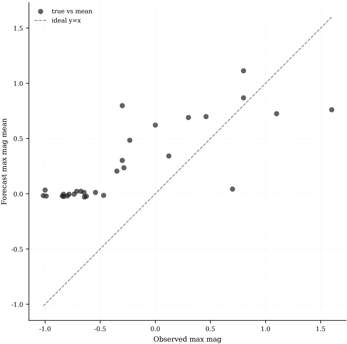
Observed vs Forecast Max Magnitude | MAE: 0.64
