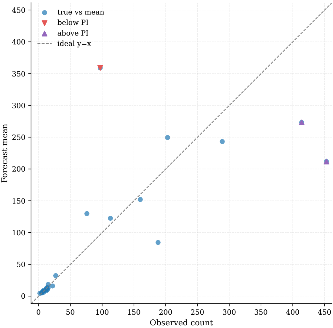
Observed vs Forecast (zoomed) | Coverage: 83.33%
