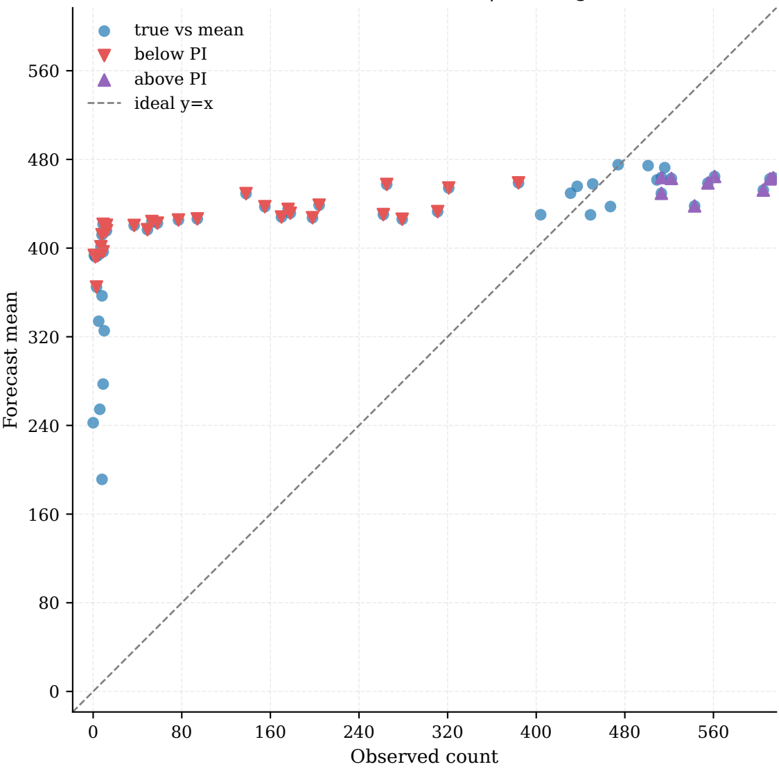
Observed vs Forecast (zoomed) | Coverage: 22.97%
