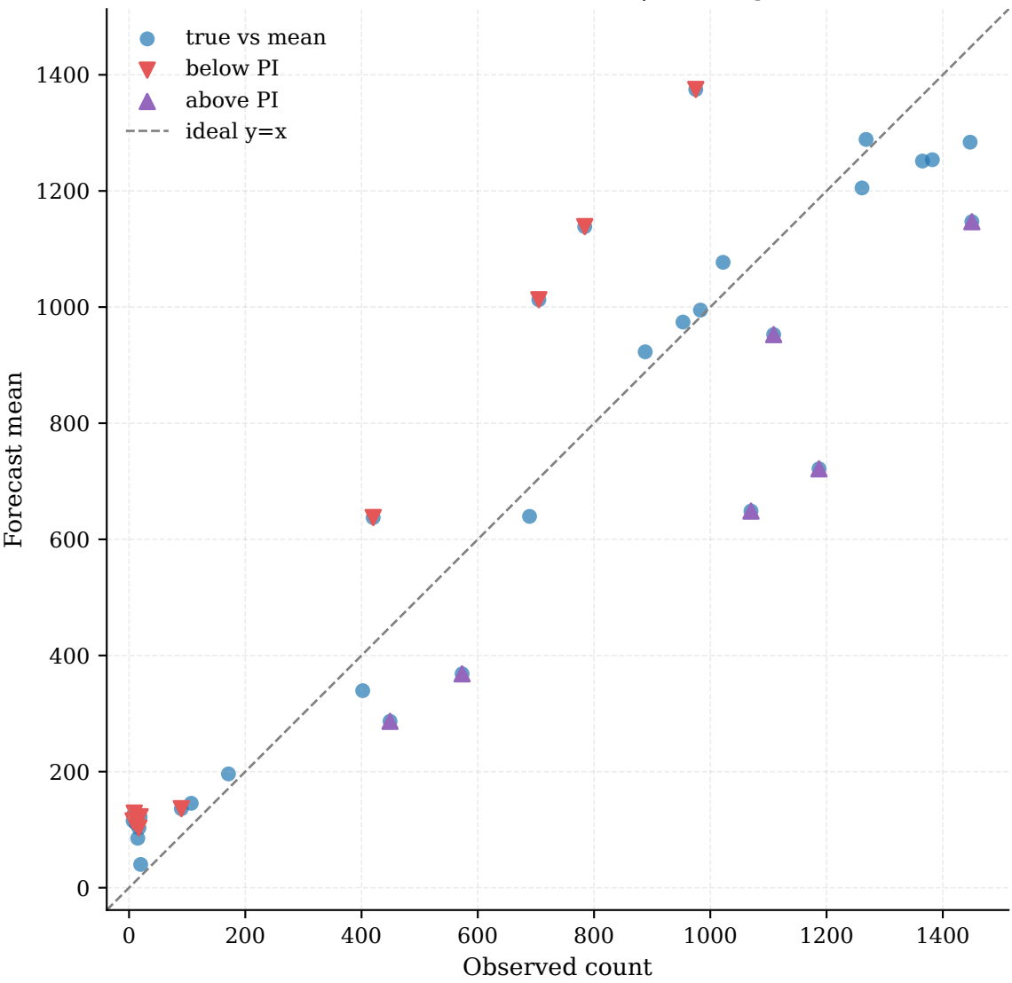
Observed vs Forecast (zoomed) | Coverage: 41.67%
