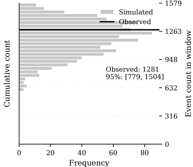
Forecast counts
