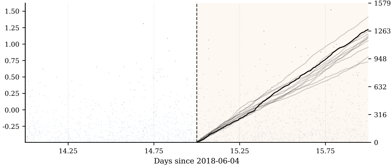
Observed Sequence and Example Forecast Trajectories
