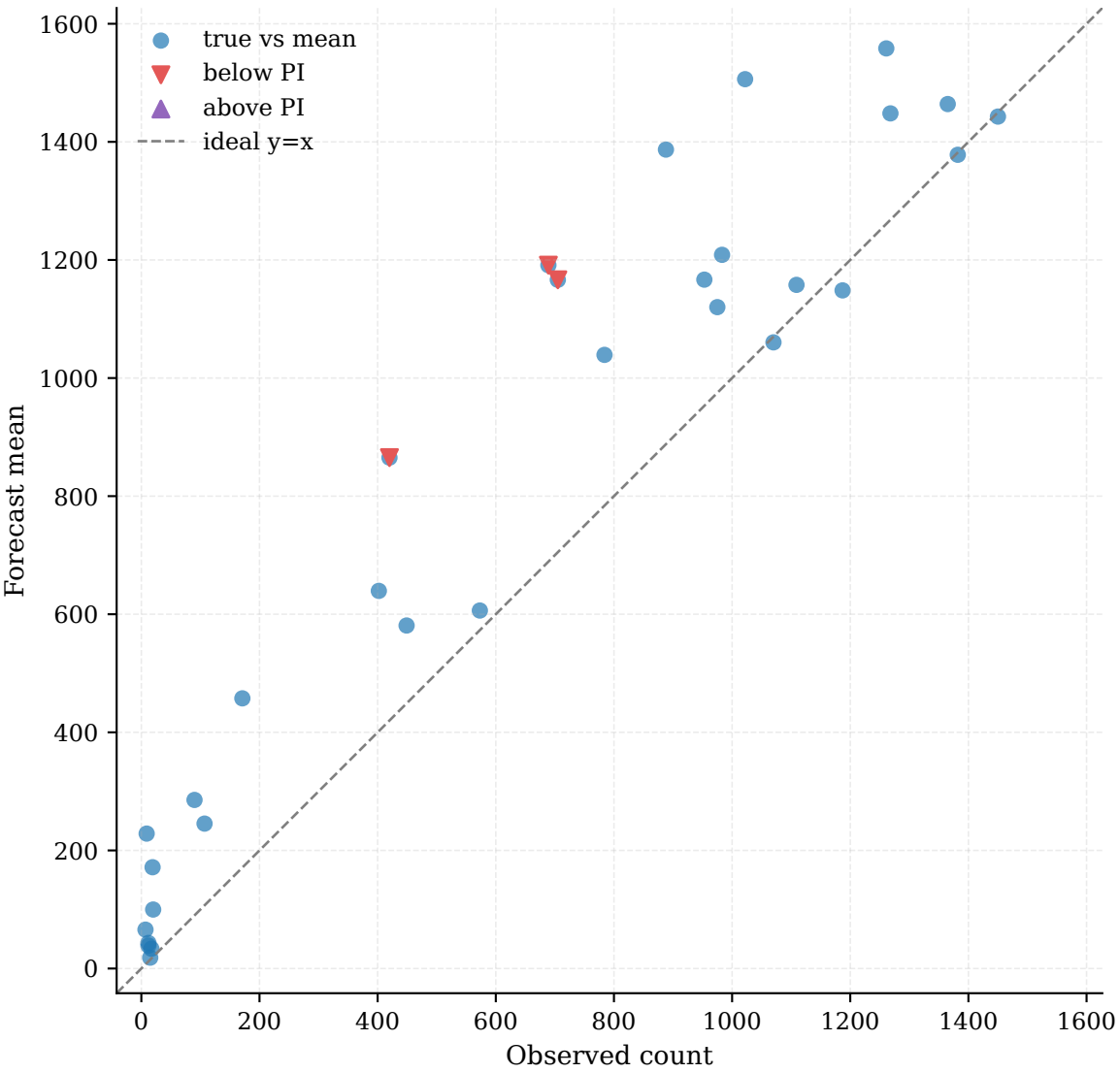
Observed vs Forecast (zoomed) | Coverage: 91.67%
