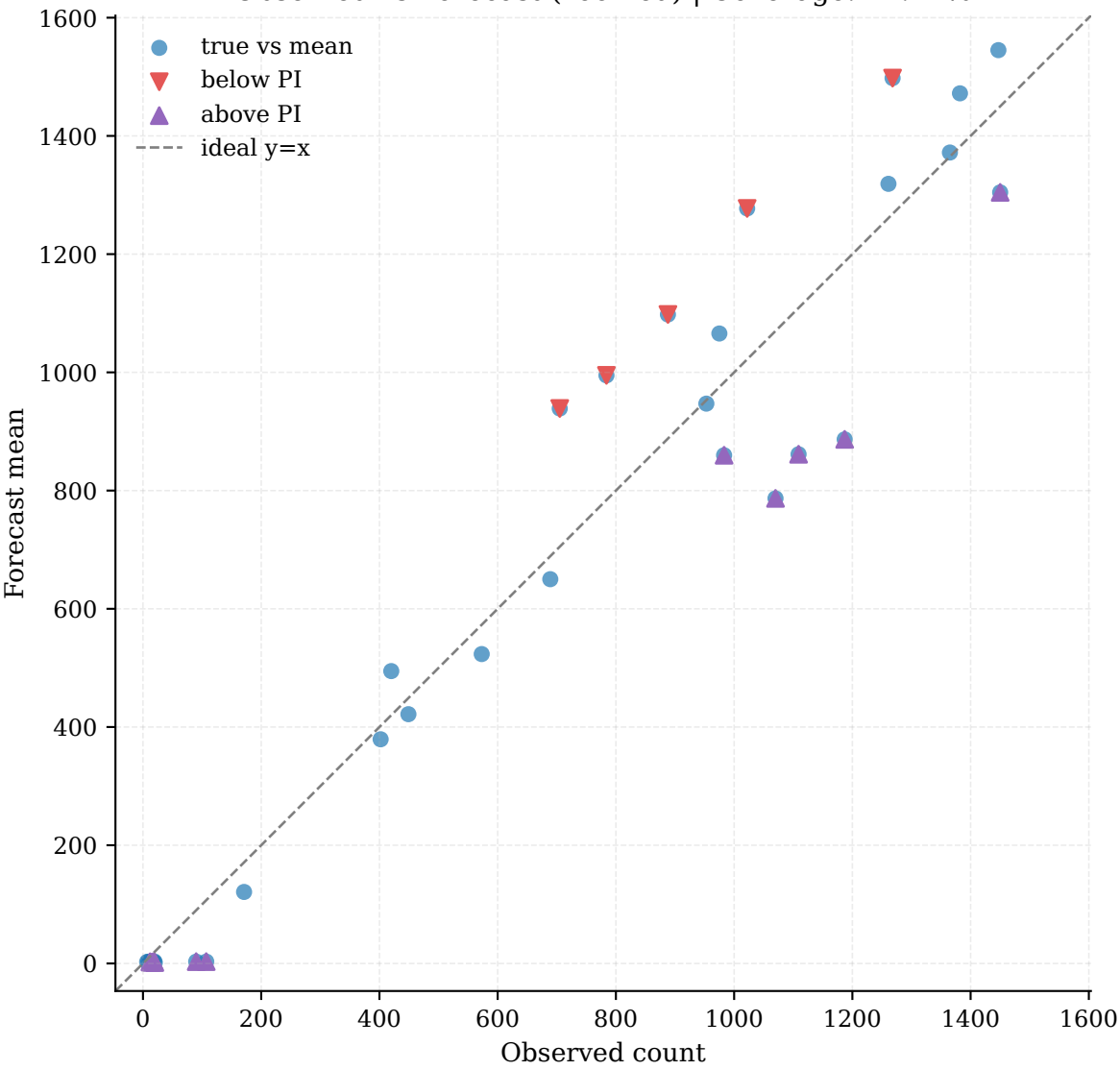
Observed vs Forecast (zoomed) | Coverage: 47.22%
