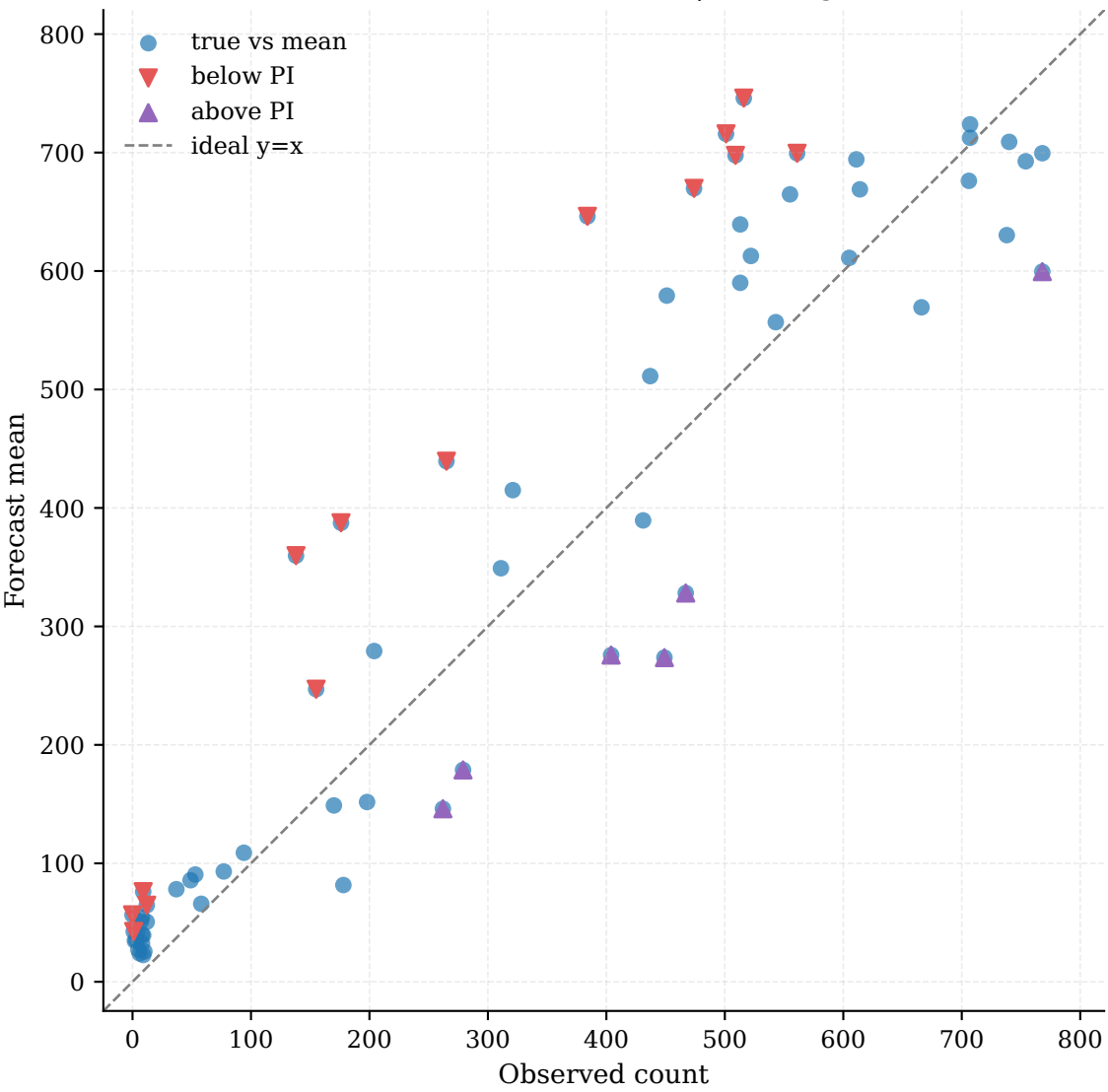
Observed vs Forecast (zoomed) | Coverage: 68.92%
