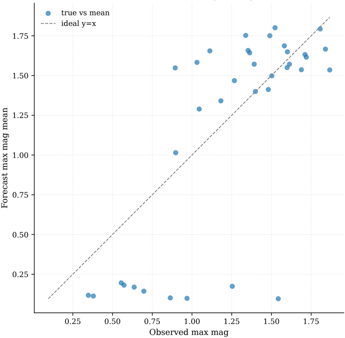
Observed vs Forecast Max Magnitude | MAE: 0.33
