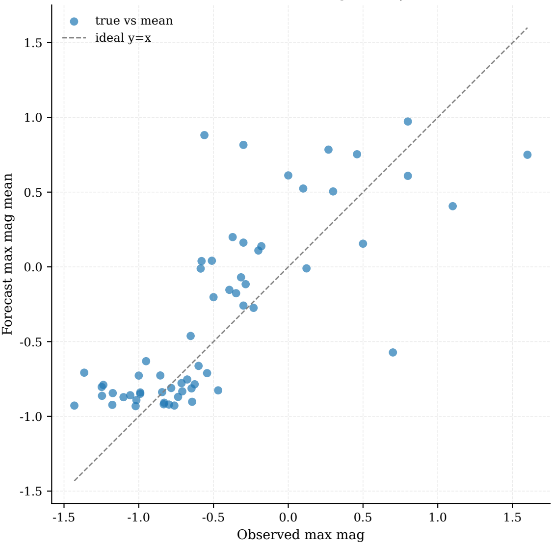
Observed vs Forecast Max Magnitude | MAE: 0.32
