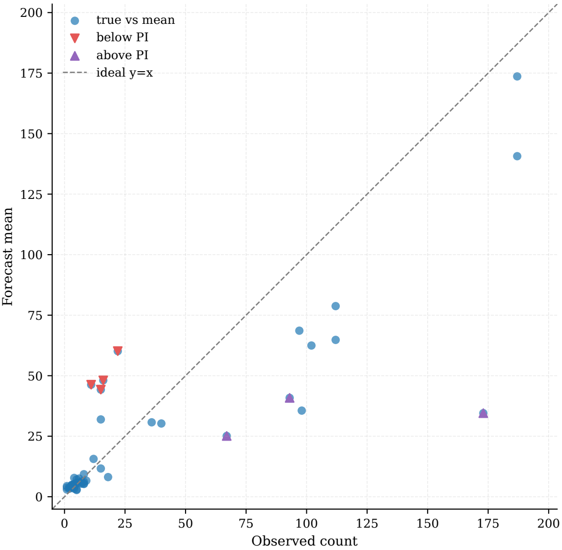
Observed vs Forecast (zoomed) | Coverage: 83.61%
