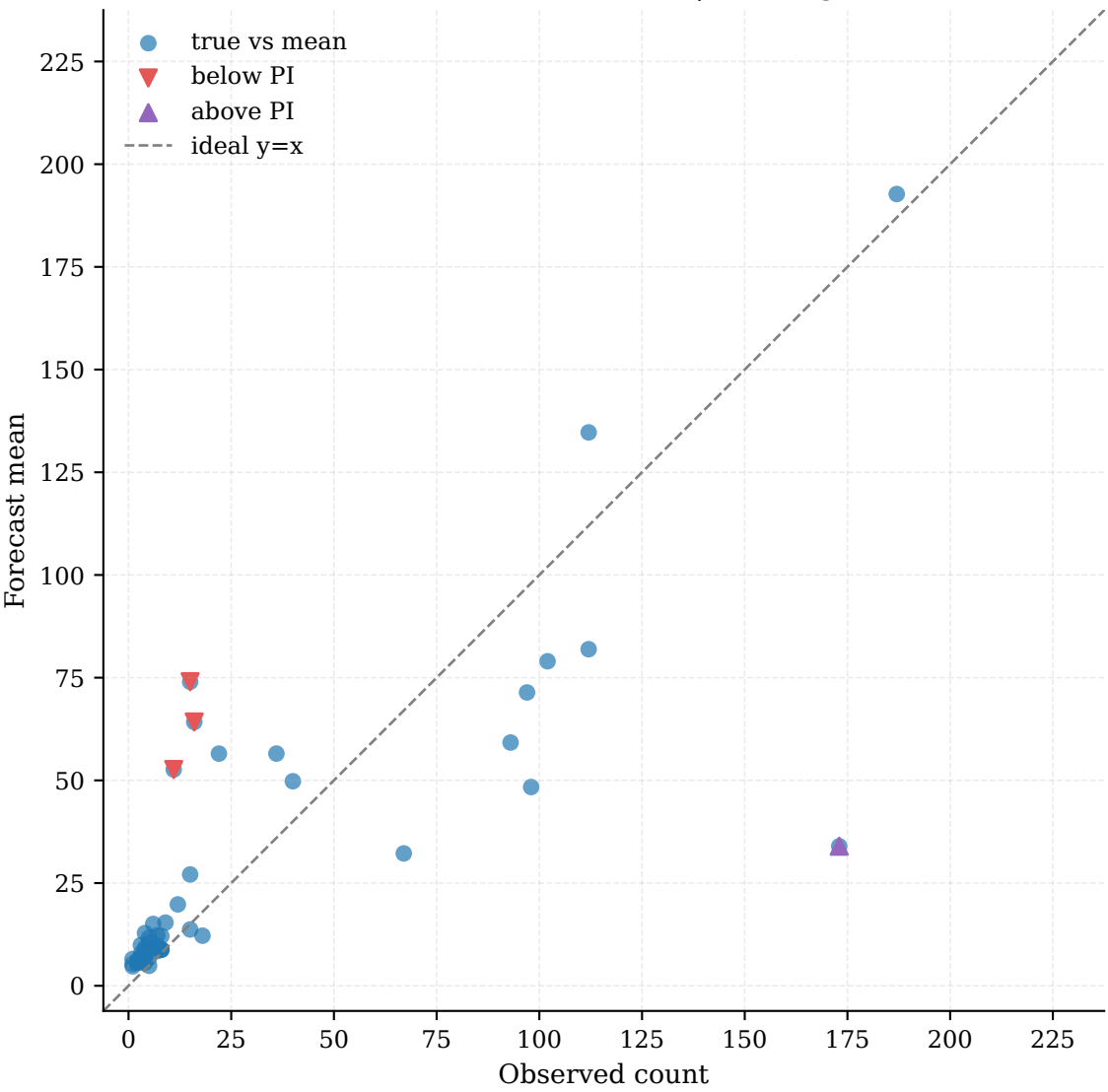
Observed vs Forecast (zoomed) | Coverage: 88.52%
