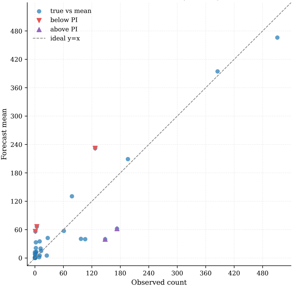
Observed vs Forecast (zoomed) | Coverage: 77.27%
