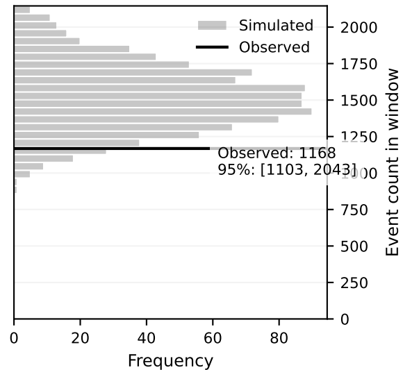
Forecast counts
