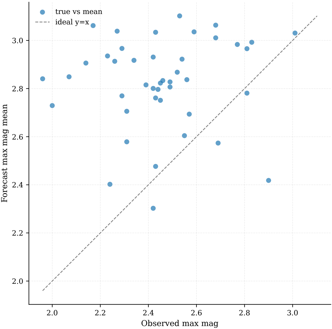
Observed vs Forecast Max Magnitude | MAE: 0.40
