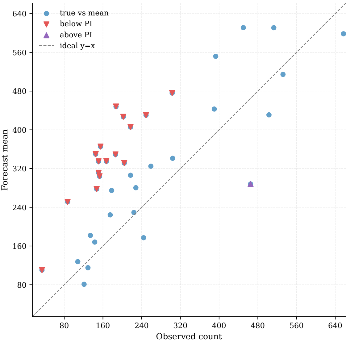
Observed vs Forecast (zoomed) | Coverage: 55.81%
