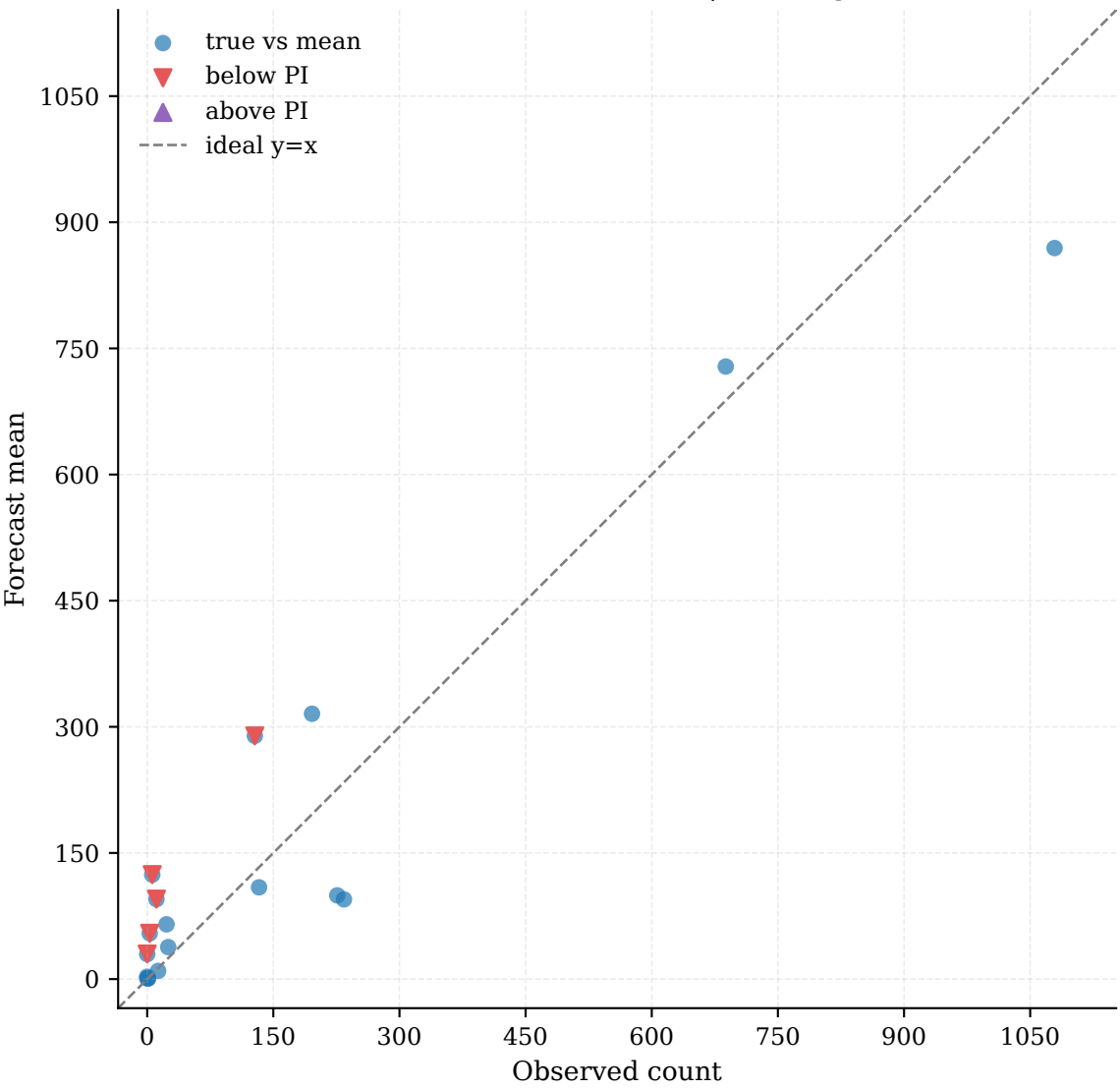
Observed vs Forecast (zoomed) | Coverage: 71.43%
