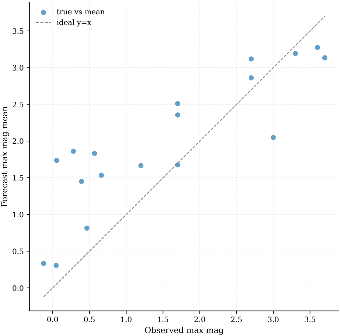
Observed vs Forecast Max Magnitude | MAE: 0.67
