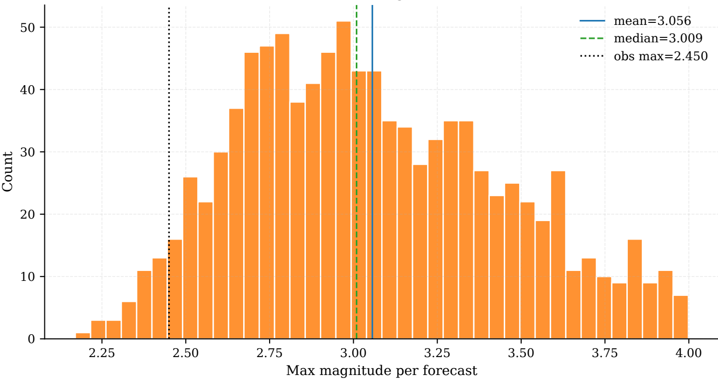
Distribution of Maximum Magnitude Across Forecasts
