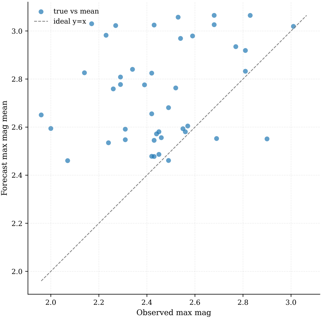
Observed vs Forecast Max Magnitude | MAE: 0.31
