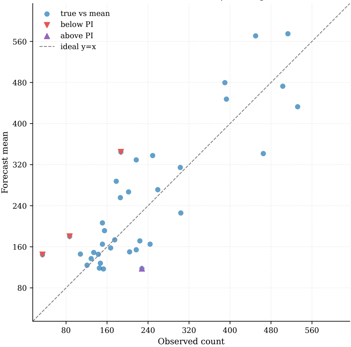
Observed vs Forecast (zoomed) | Coverage: 88.37%
