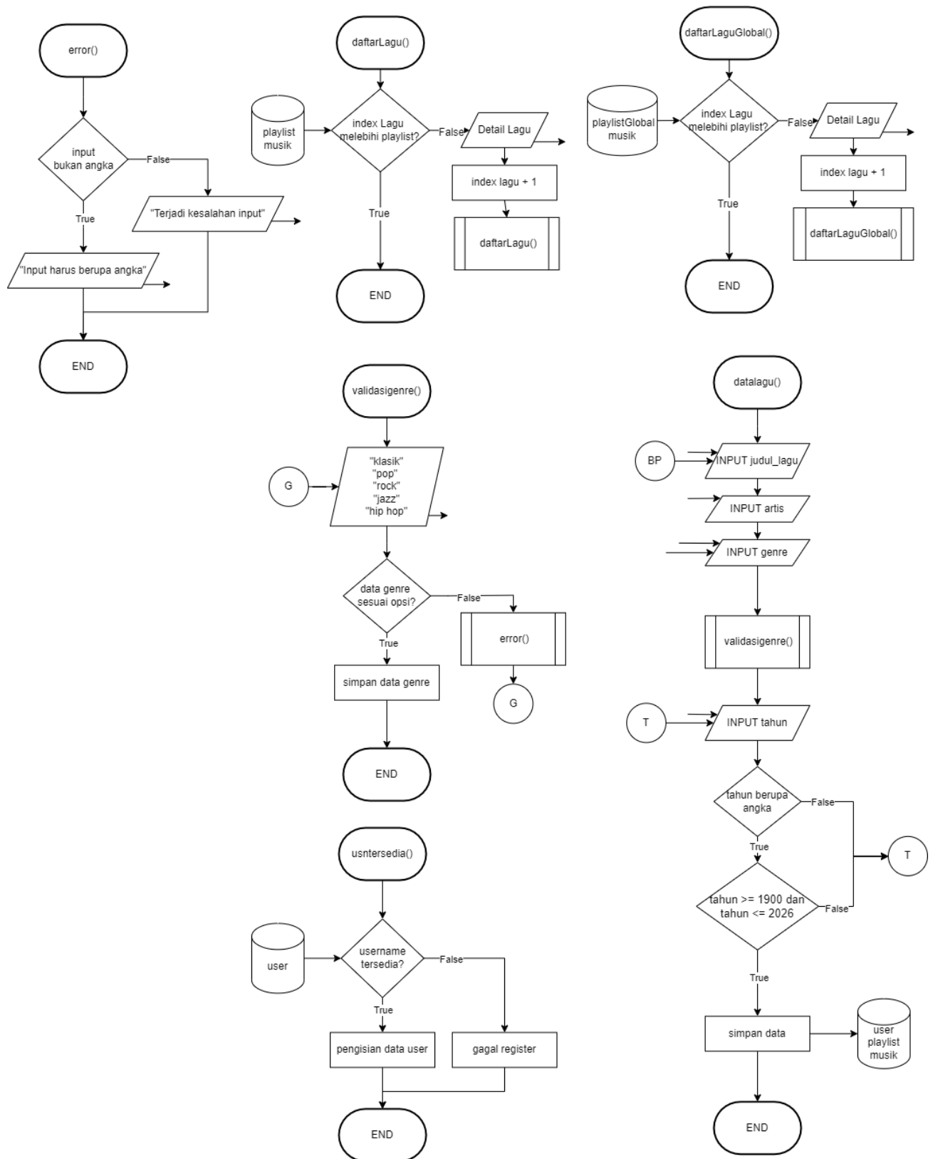
Gambar 2.12 Flowchart Fungsi Utilitas
