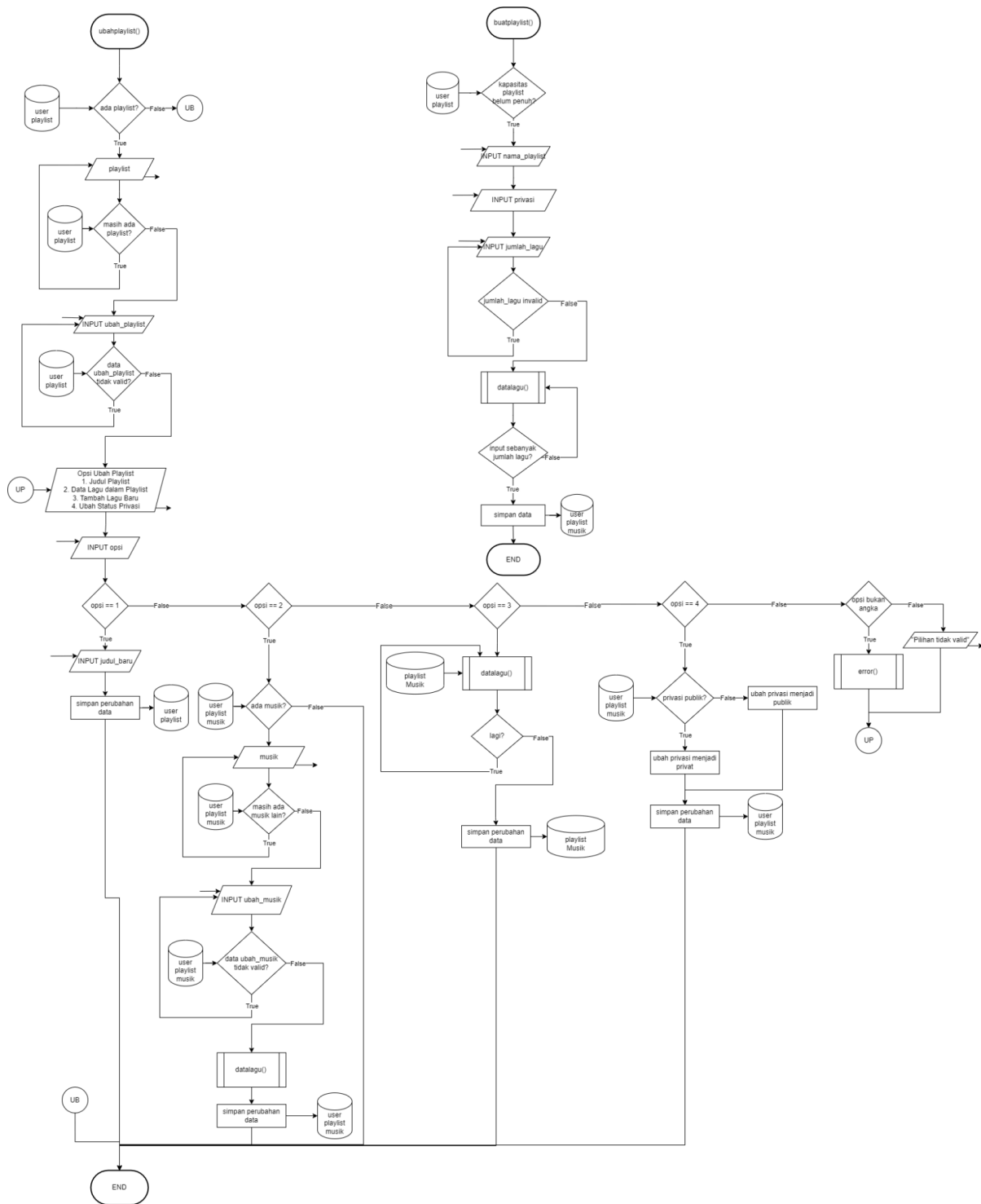
Gambar 2.7 Flowchart Fungsi Ubah & Buat Playlist
