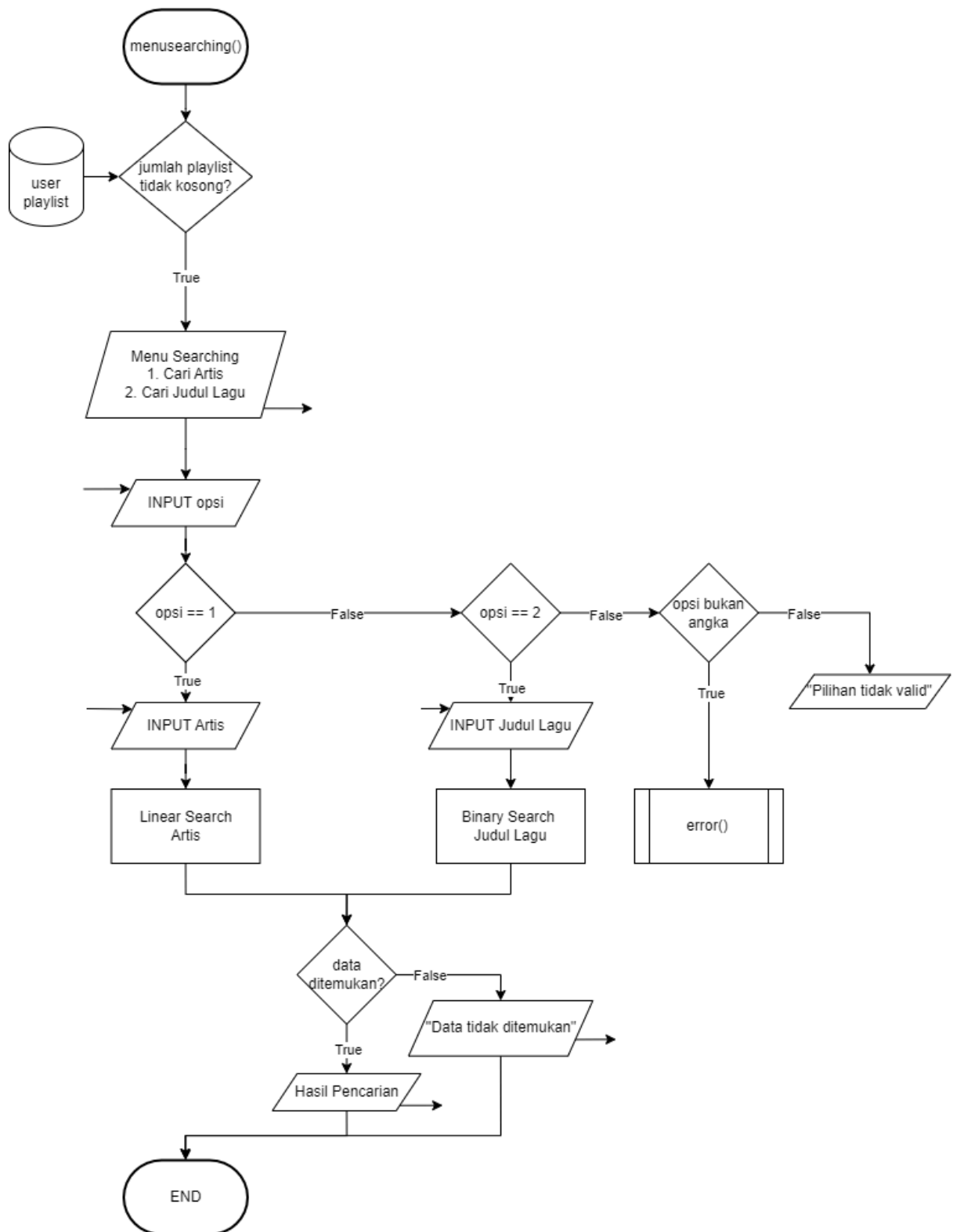
Gambar 2.11 Flowchart Menu Searching
