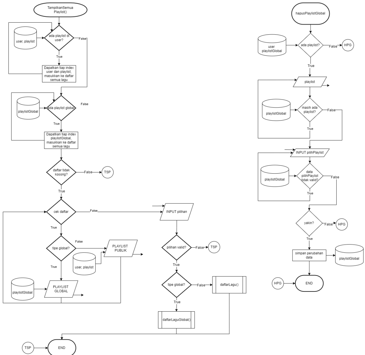
Gambar 2.5 Flowchart Fungsi Lihat semua playlist & Hapus Playlist Global
