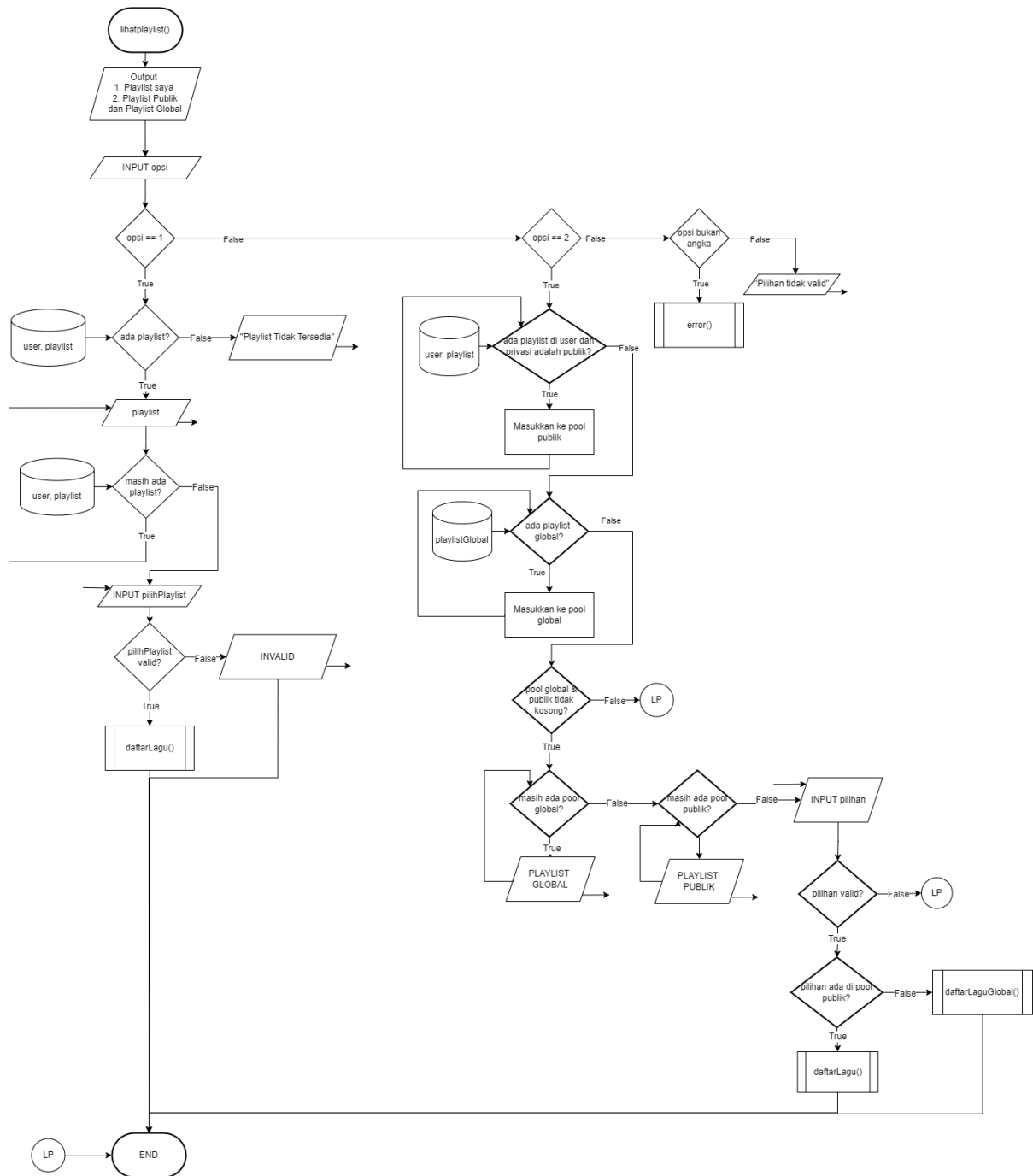
Gambar 2.8 Flowchart Fungsi Lihat Playlist
