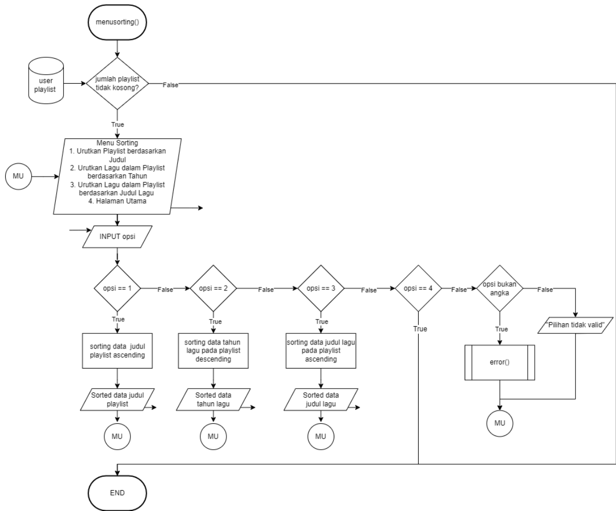
Gambar 2.10 Flowchart Menu Sorting
