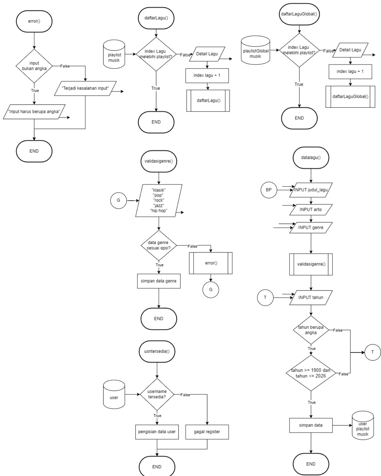
Gambar 2.12 Flowchart Fungsi Utilitas
